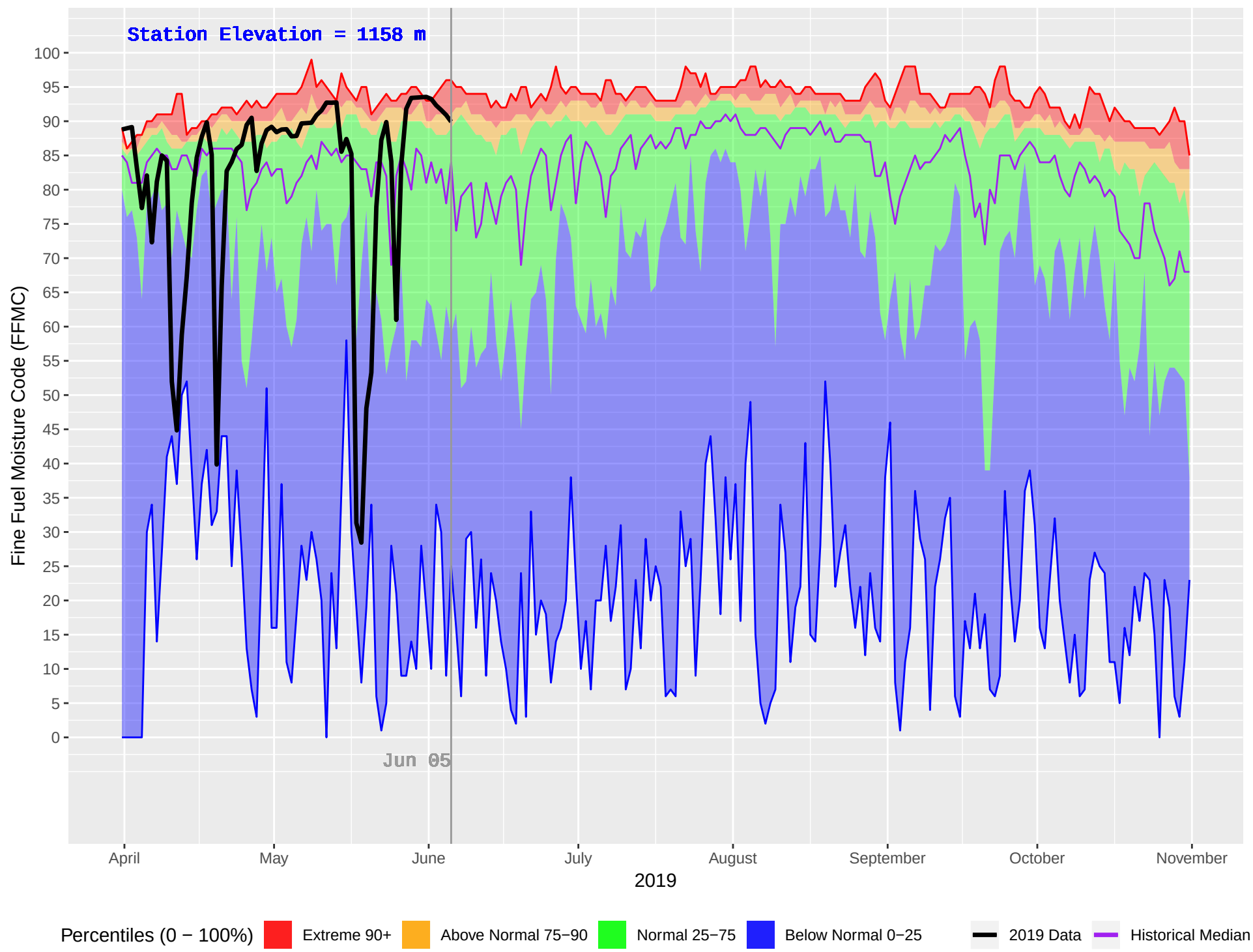
LONE BUTTE (218) : Historical (1987–2018) and Current (2019) Daily Fine Fuel Moisture Code (FFMC)
