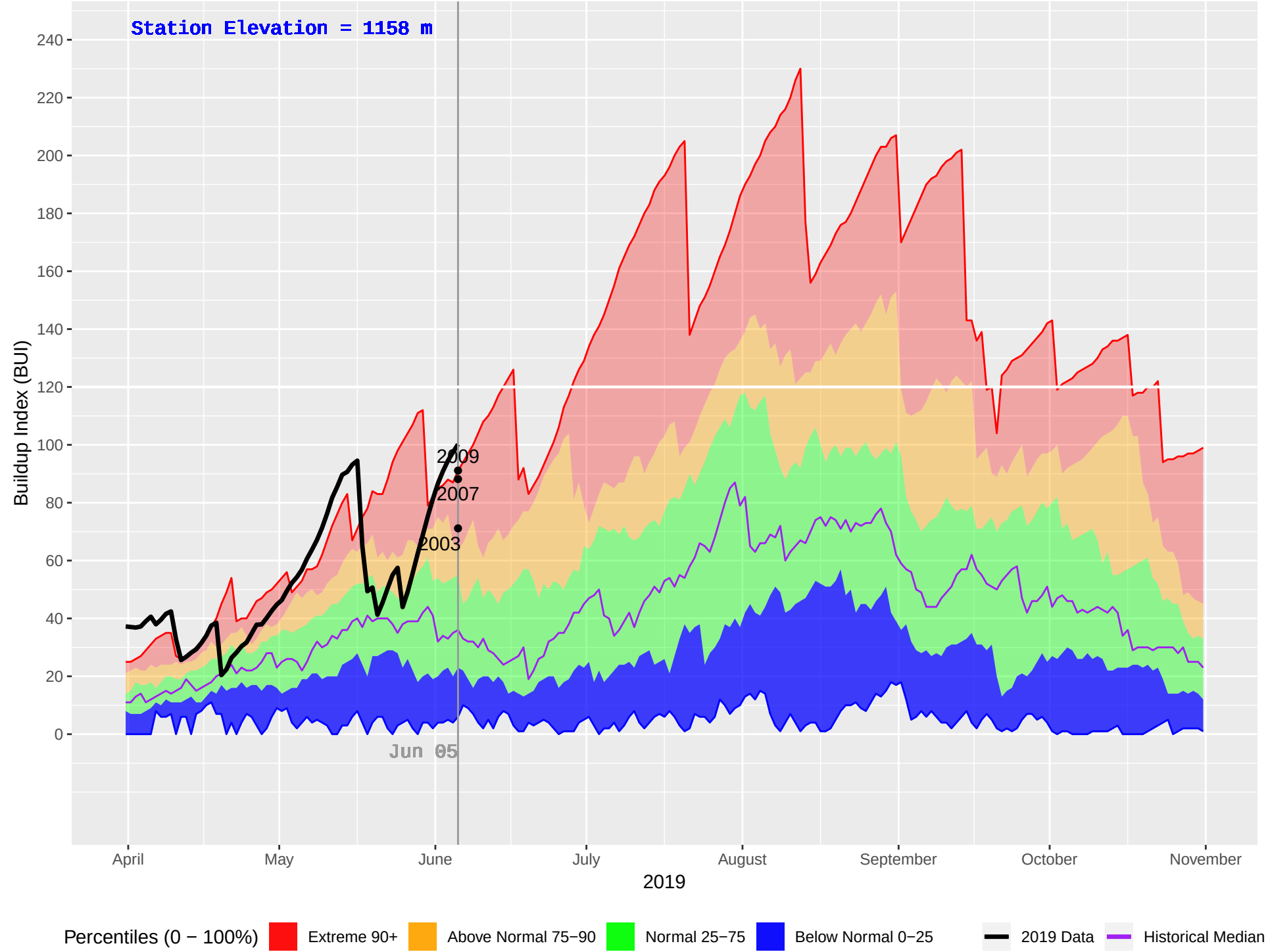
LONE BUTTE (218) : Historical (1987–2018), Current (2019) Daily Buildup Index (BUI)
