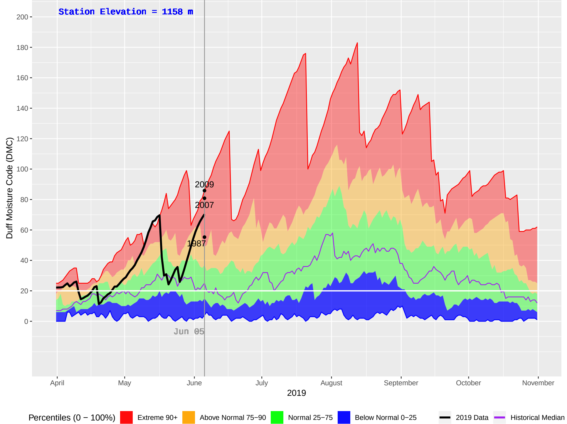
LONE BUTTE (218) : Historical (1987–2018), Current (2019) Daily Duff Moisture Code (DMC)
