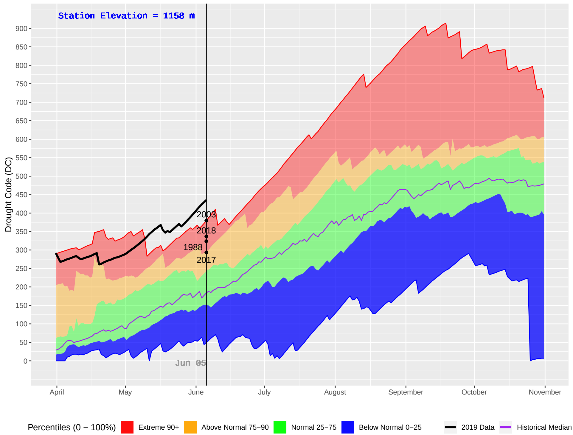
LONE BUTTE (218) : Historical (1987–2018) and Current (2019) Daily Drought Code (DC)
