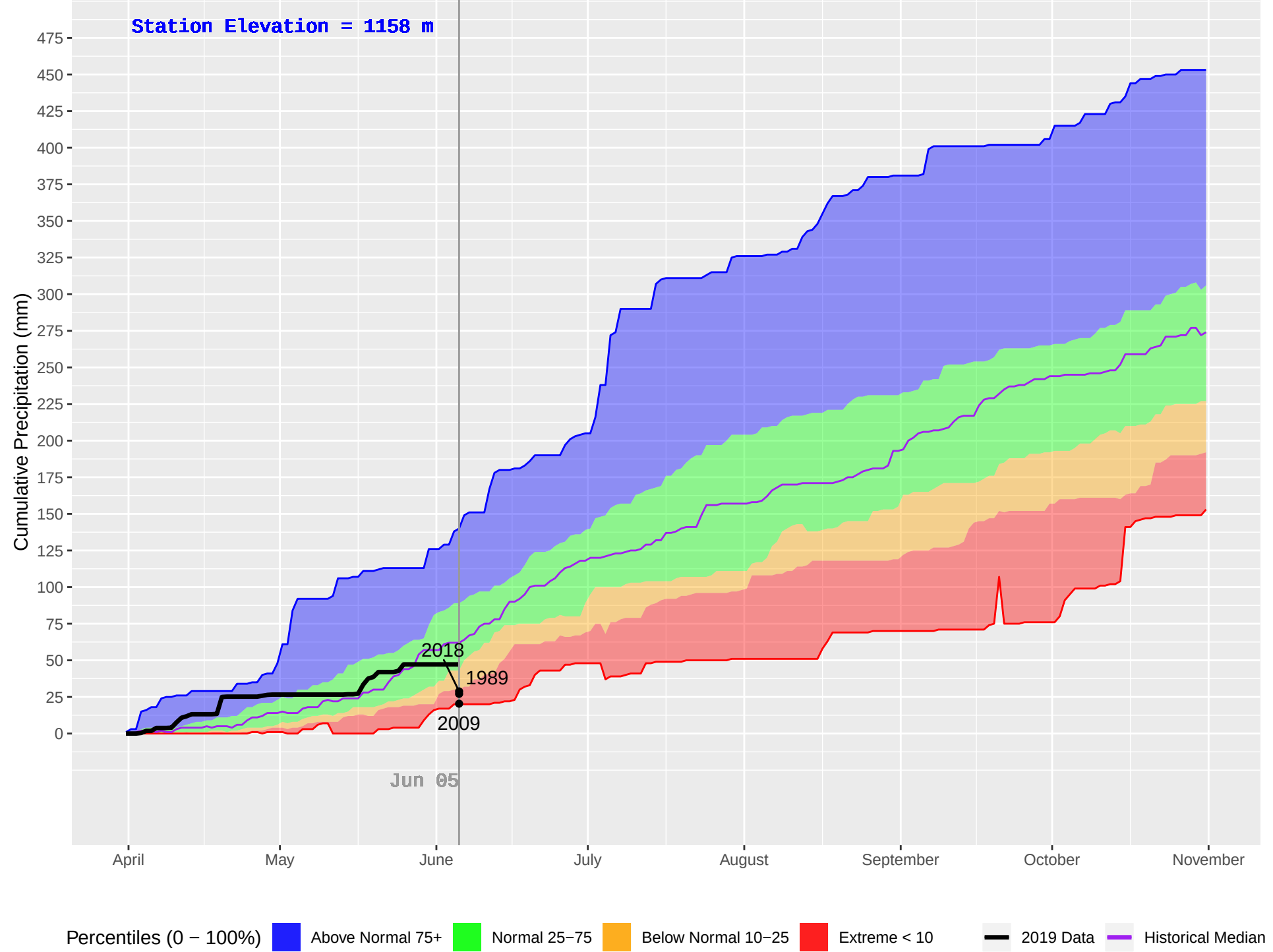
LONE BUTTE (218) : Historical (1987–2018), Current (2019) Daily Cumulative Precipitation
