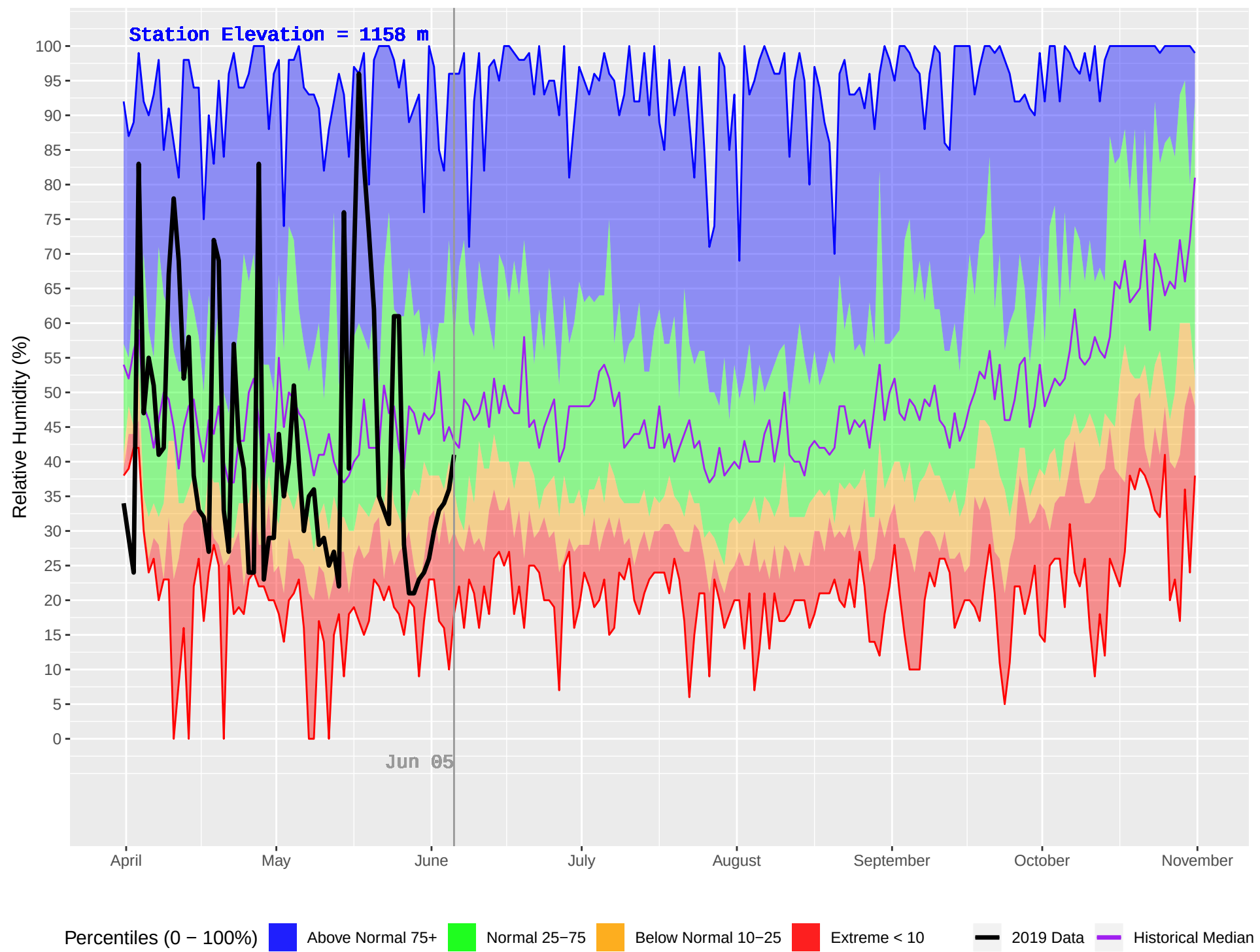
LONE BUTTE (218) : Historical (1987–2018) and Current (2019) Daily Relative Humidity
